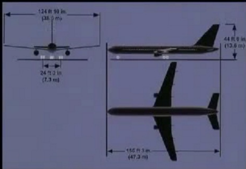
Figure 3.1 Dimensions of Boeing 757-200 aircraft
